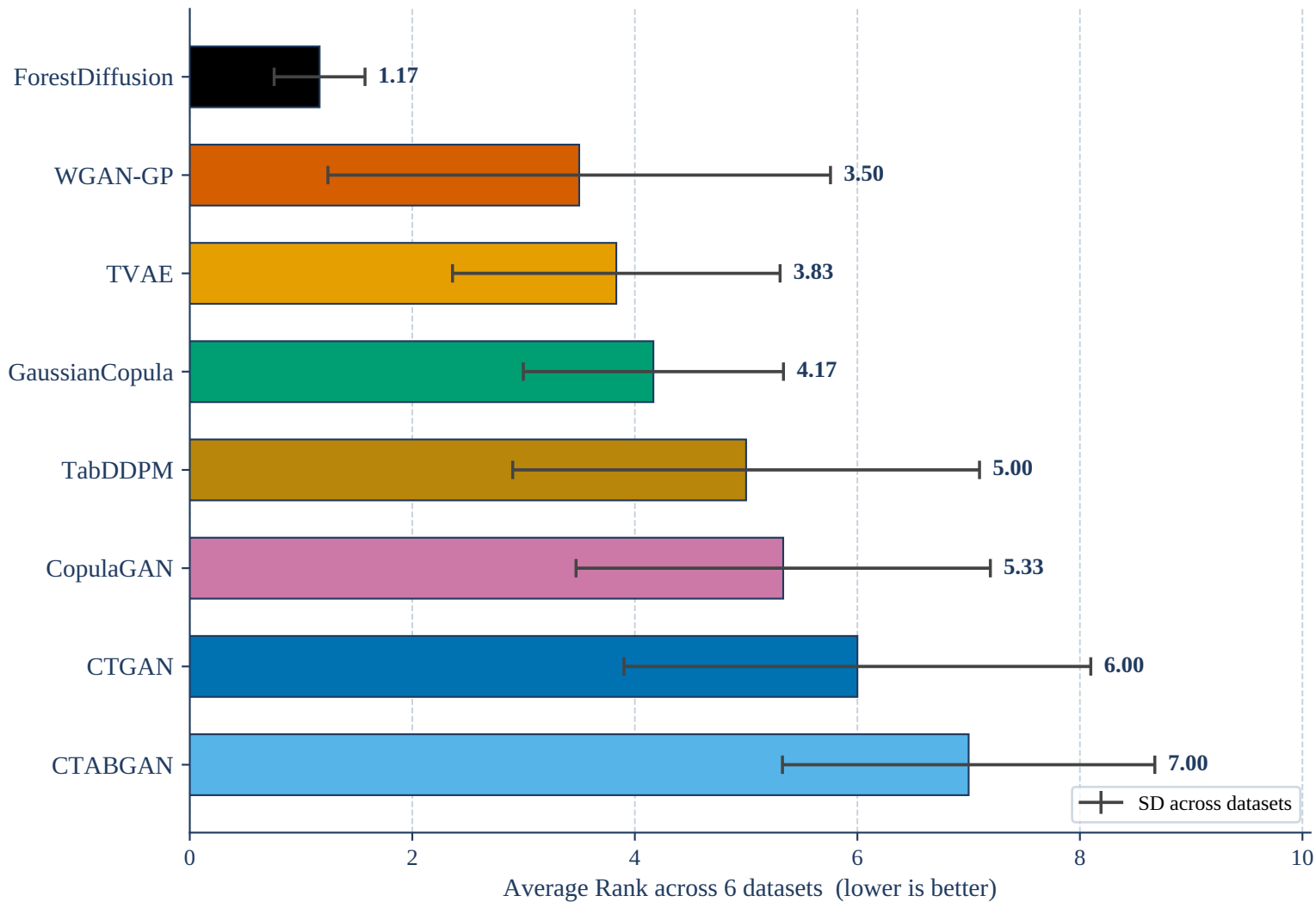
Generator Robustness — Average R^2 -Gap Rank (10-seed means)
